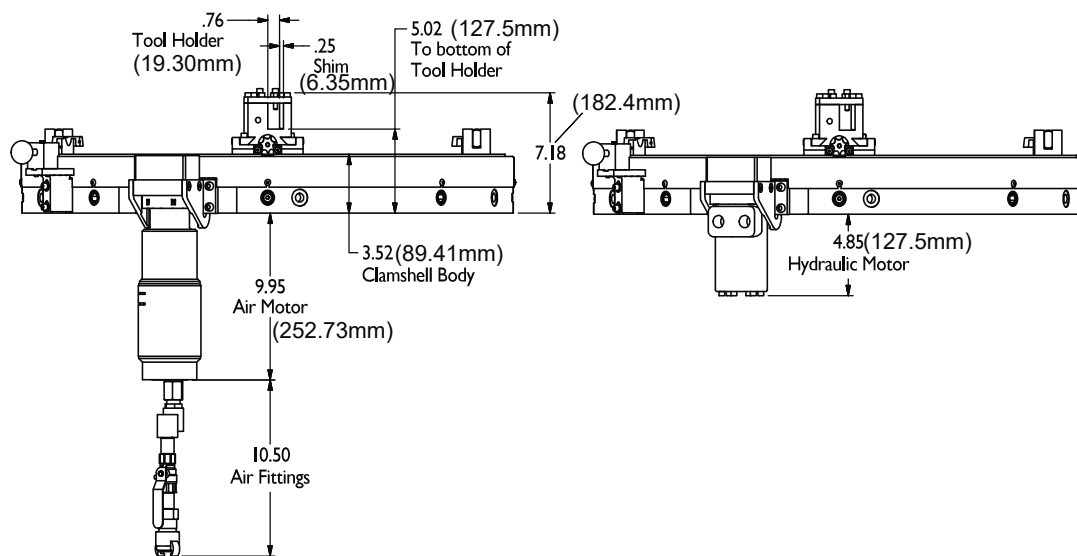
USS CLAMSHELL PORTABLE LATHE DIMENSIONS
