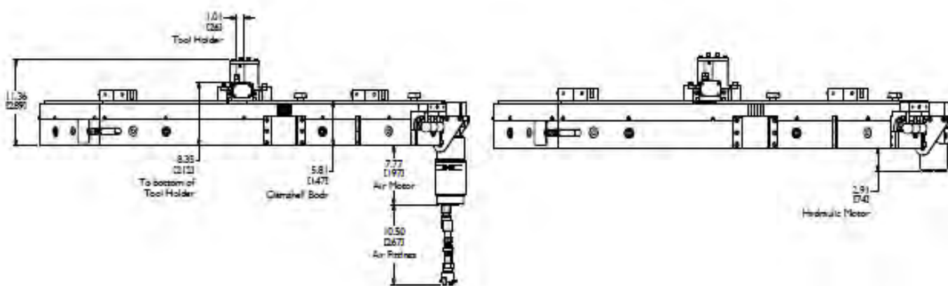
WD CLAMSHELL PORTABLE LATHE DIMENSIONS
