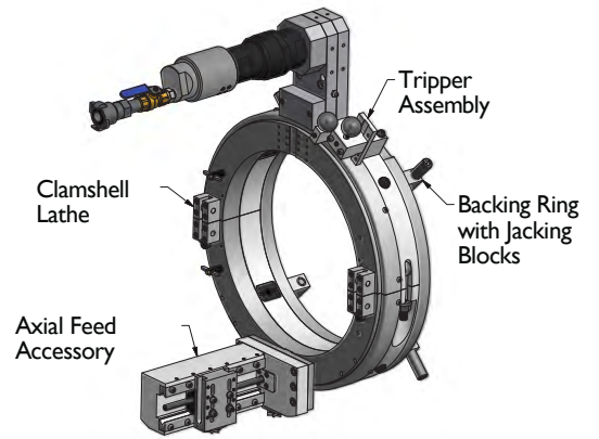
Axial Feed Accessory and Backing Ring
